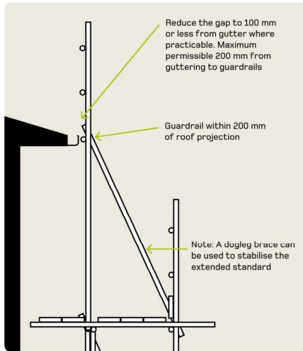
Figure 9: The use of scaffolding for edge protection.
